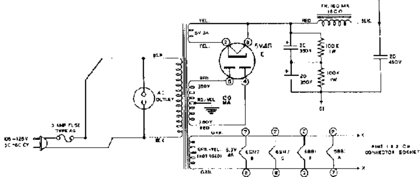
HEATHKIT WILLIAMSON-TYPE AMPLIFIER
